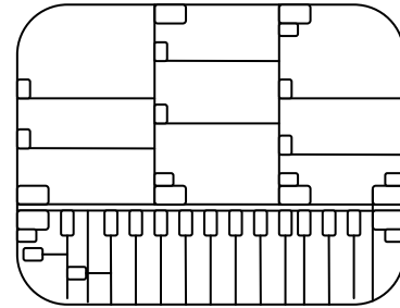
THC-3 87046 Standard Tray with Ampule Dividers 21-1/2"W x 15-1/4"D x 2-5/16"H
